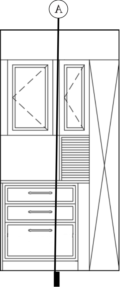
PANTRY ELEVATION
