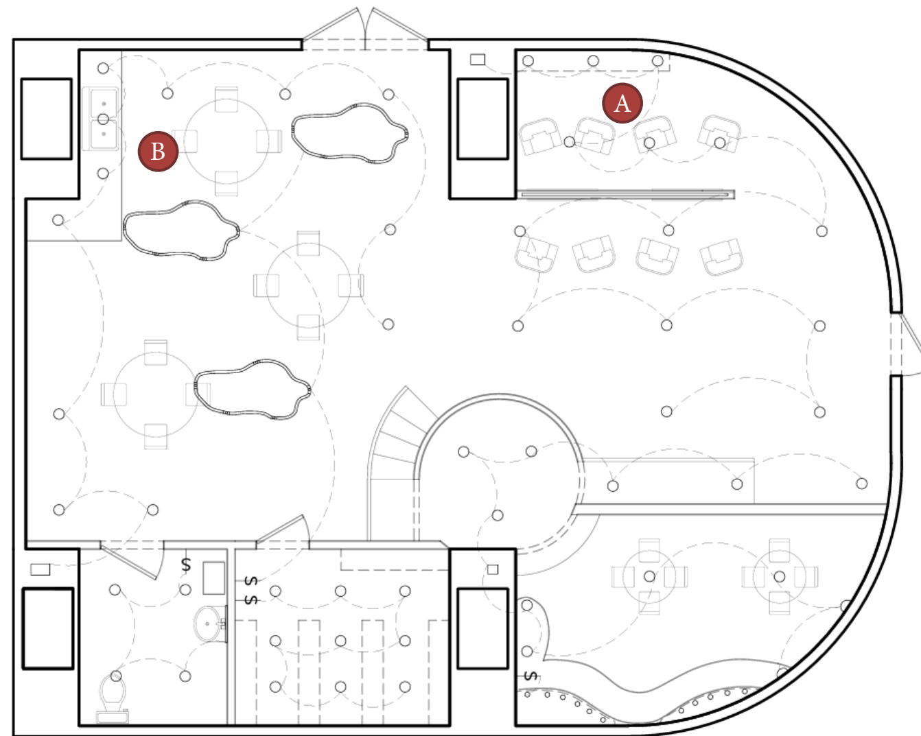
LIGHTING PLAN
