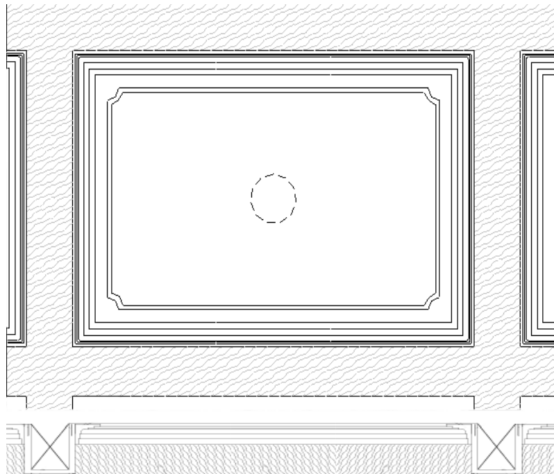
COFFERED CEILING
