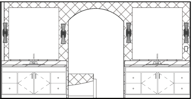
BOYS' BATHROOM
