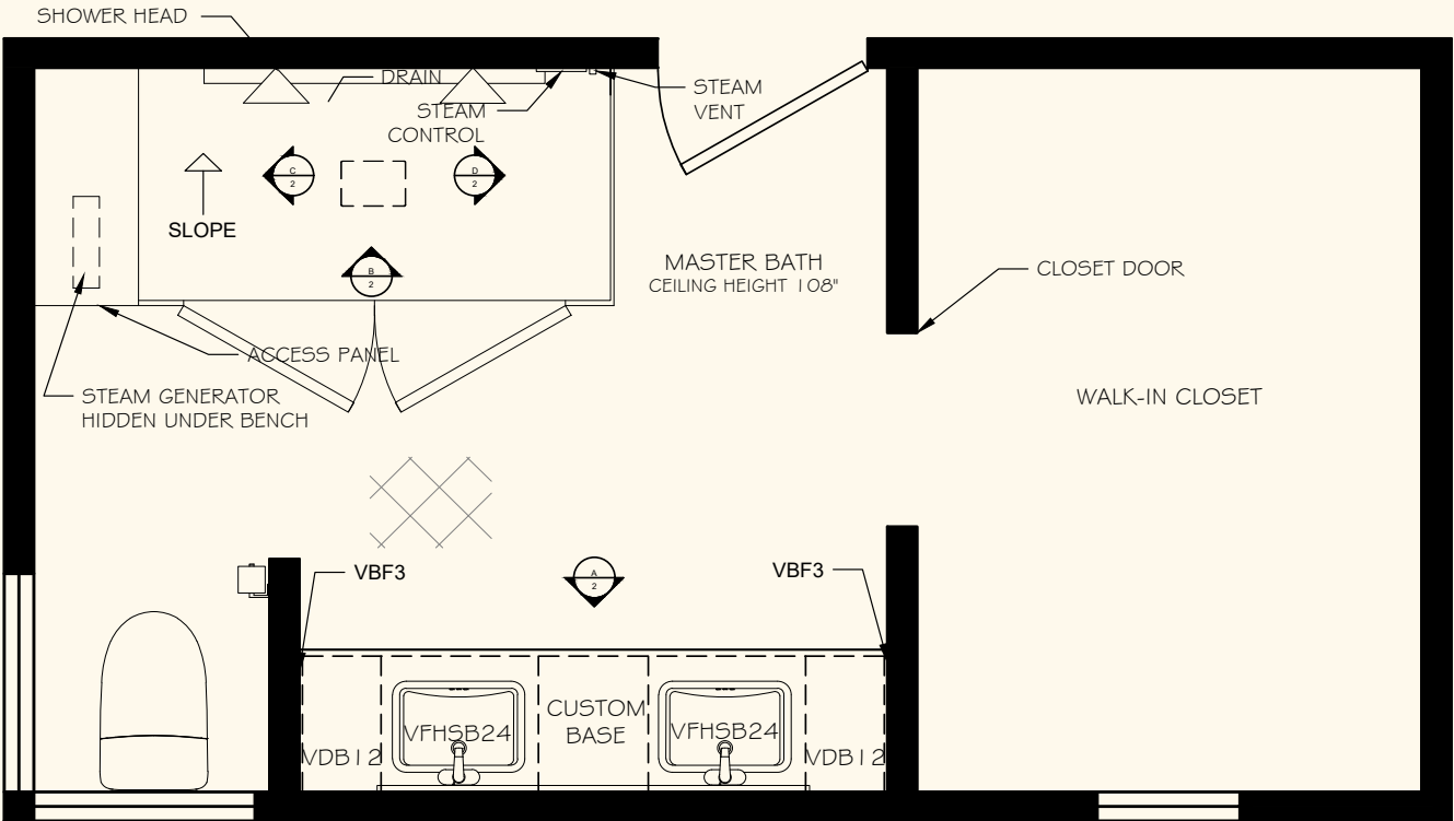
AFTER PLAN
