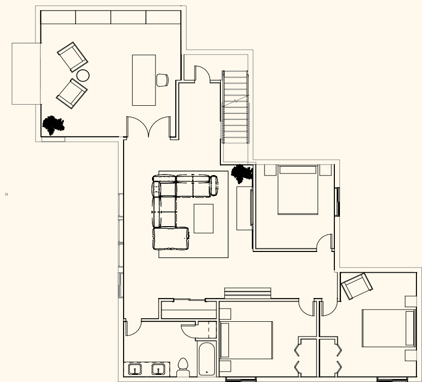
FINAL PLAN BASEMENT
