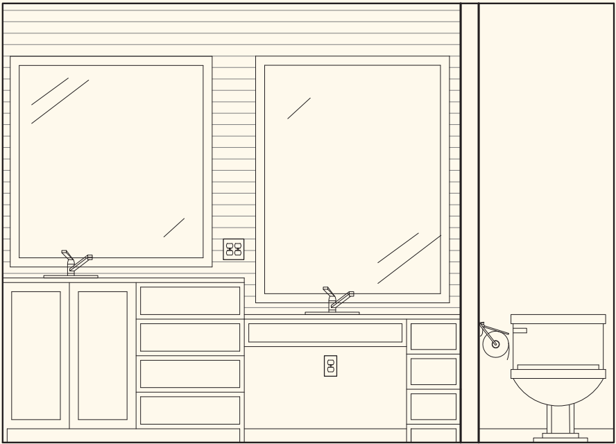
MASTER BATH ELEVATION
