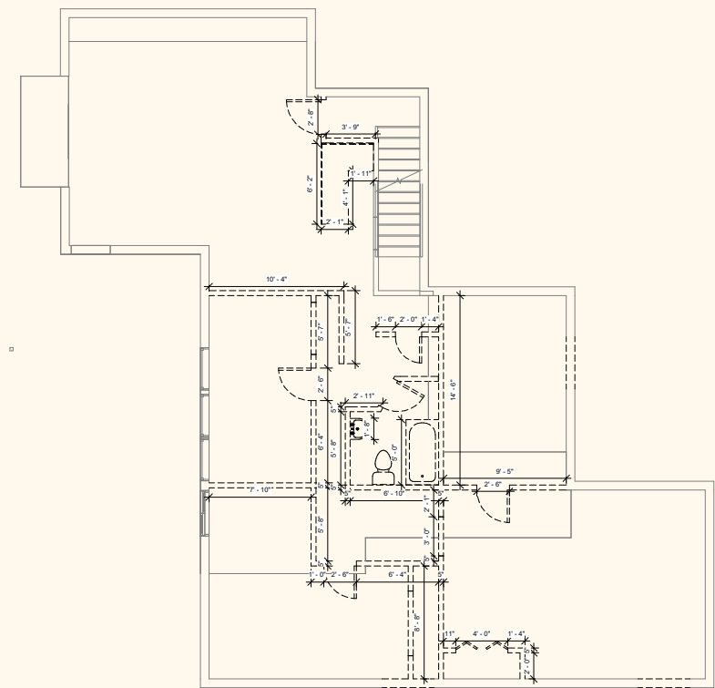
DEMO PLAN BASEMENT
