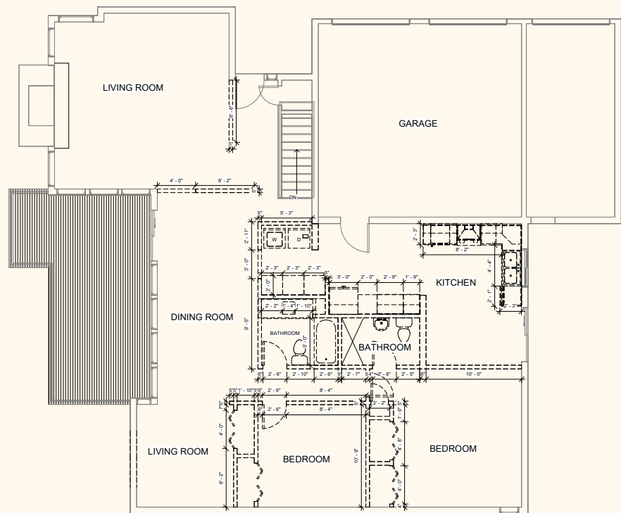
DEMO PLAN MAIN FLOOR
