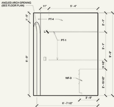
5 MASTER CLOSET 1 ELEVATION 1/2" = 1'-0"
