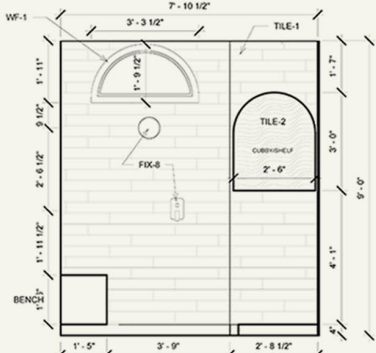
2 MASTER BATHROOM SHOWER ELEVATION 1/2" = 1'-0"
