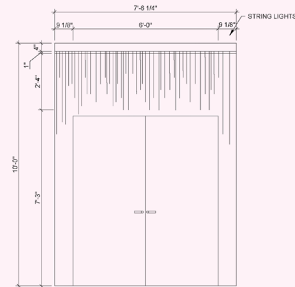
1 A9 - MAIN ENTRANCE ELEVATION SCALE: 1/2" = 1'-0"
