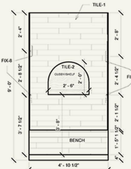
1 MASTER BATHROOM SHOWER ELEVATION 1/2" = 1'-0"
