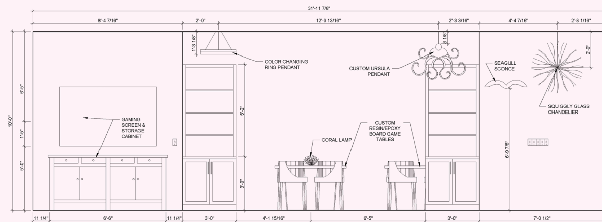
1 A8 - SOUTH MIDDLE END WALL ELEVATION SCALE: 1/2" = 1'-0" 1 A8 - BOARD GAME TABLE ELEVATION SCALE: 1/2" = 1'-0" 1 A8 - NORTH MIDDLE END WALL ELEVATION SCALE: 1/2" = 1'-0"
