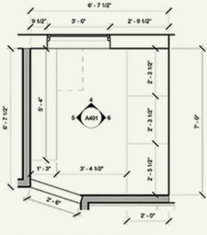
MC ENLARGED MASTER CLOSET 1 PLAN 1/2" = 1'-0"
