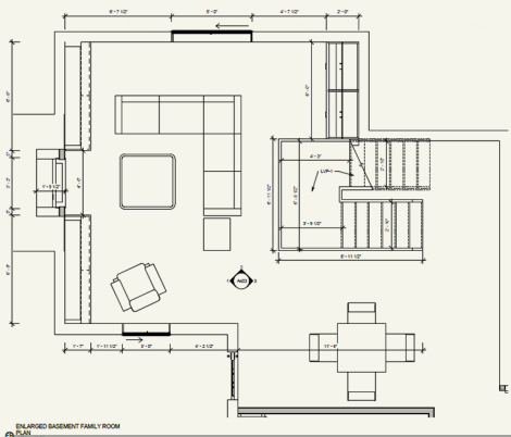
ENLARGED BASEMENT FAMILY ROOM PLAN 1/2" = 1'-0"
