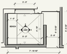
ENLARGED MASTER BATHROOM SHOWER PLAN 1/2" = 1'-0"
