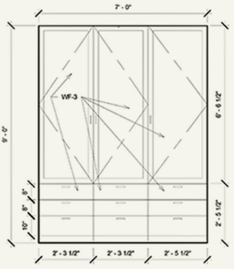
6 MASTER CLOSET 1 ELEVATION 1/2" = 1'-0"
