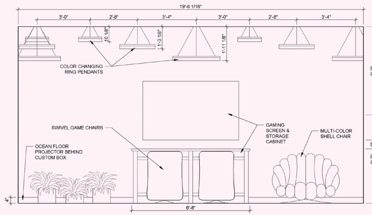
2 A7 - NORTHEAST WALL ELEVATION SCALE: 1/2" = 1'-0"
