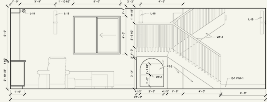
2 BASEMENT FAMILY ROOM ELEVATION 1/2" = 1'-0"
