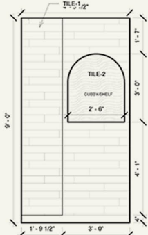
3 MASTER BATHROOM SHOWER ELEVATION 1/2" = 1'-0"
