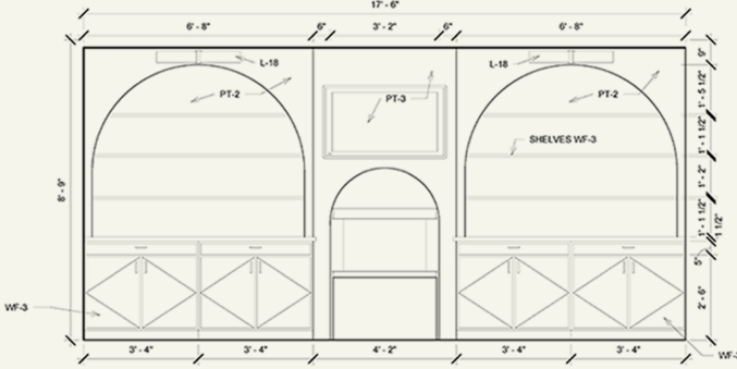
1 BASEMENT FAMILY ROOM ELEVATION 1/2" = 1'-0"
