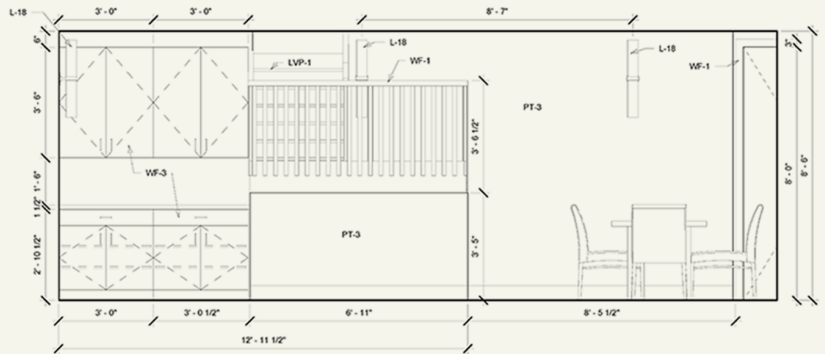
3 BASEMENT FAMILY ROOM ELEVATION 1/2" = 1'-0"
