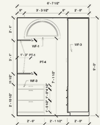
4 MASTER CLOSET 1 ELEVATION 1/2" = 1'-0"
