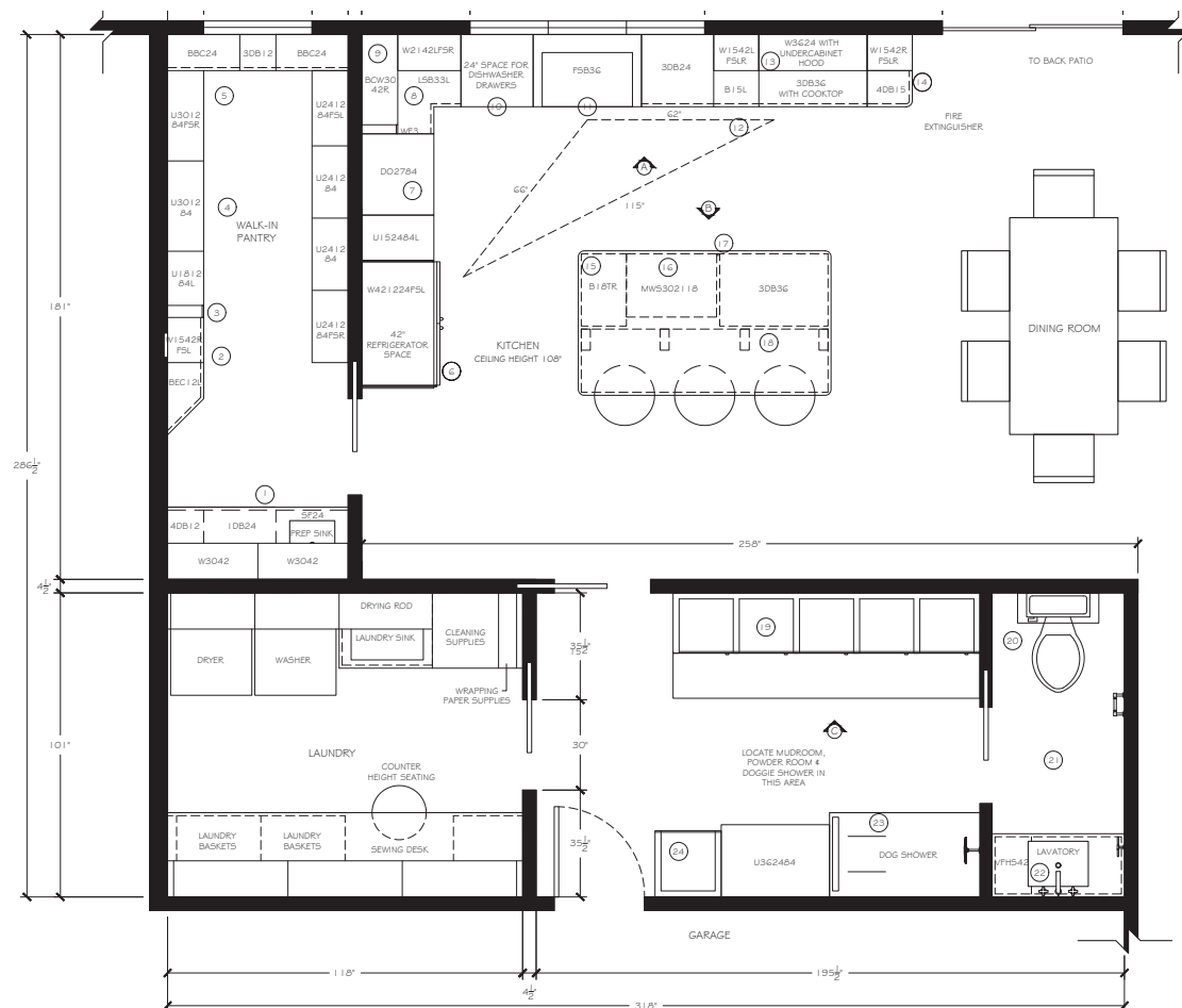
DETAILED FLOOR PLAN
