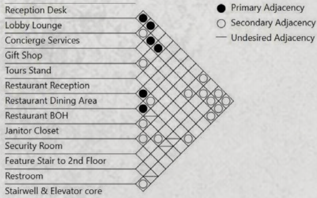
KINETIC HOTEL 1ST FLOOR ADJACNECY MATRIX LOBBY AND REESTAURANT
