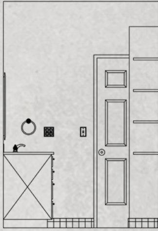
3 BATHROOM EAST ELEVATION
