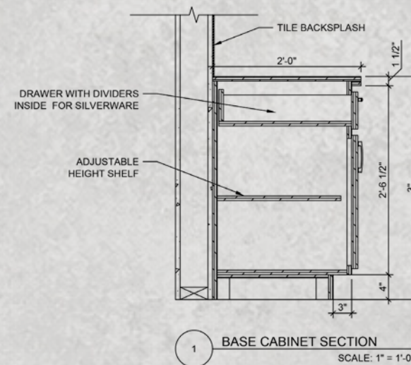
KITCHEN MADE IN AUTOCAD, RENDERED IN PHOTOSHOP
