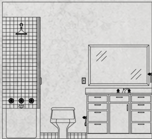
2 BATHROOM NORTH ELEVATION
