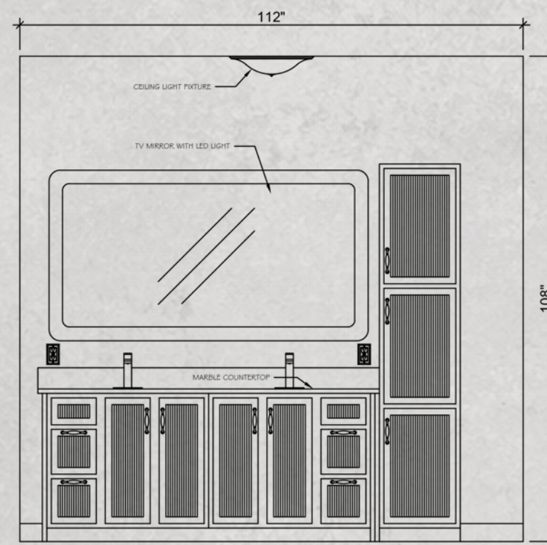
B EAST ELEVATION
