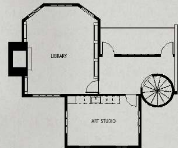
New Plan - Upper Level
