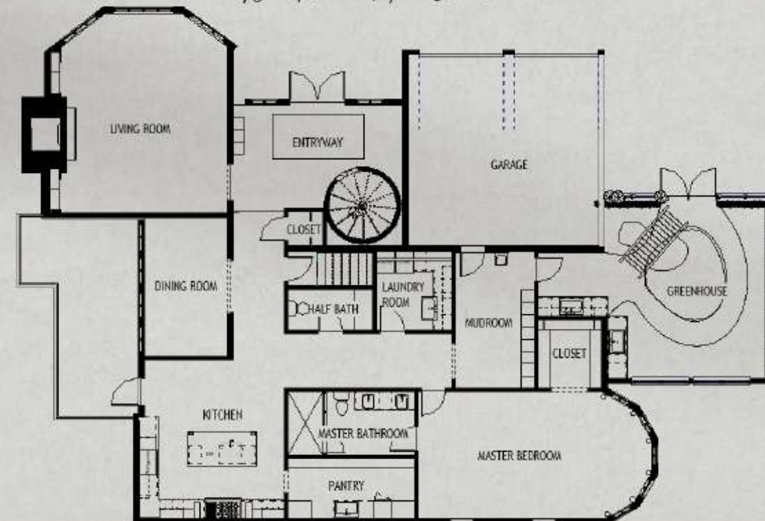
New Plan - Main Level
