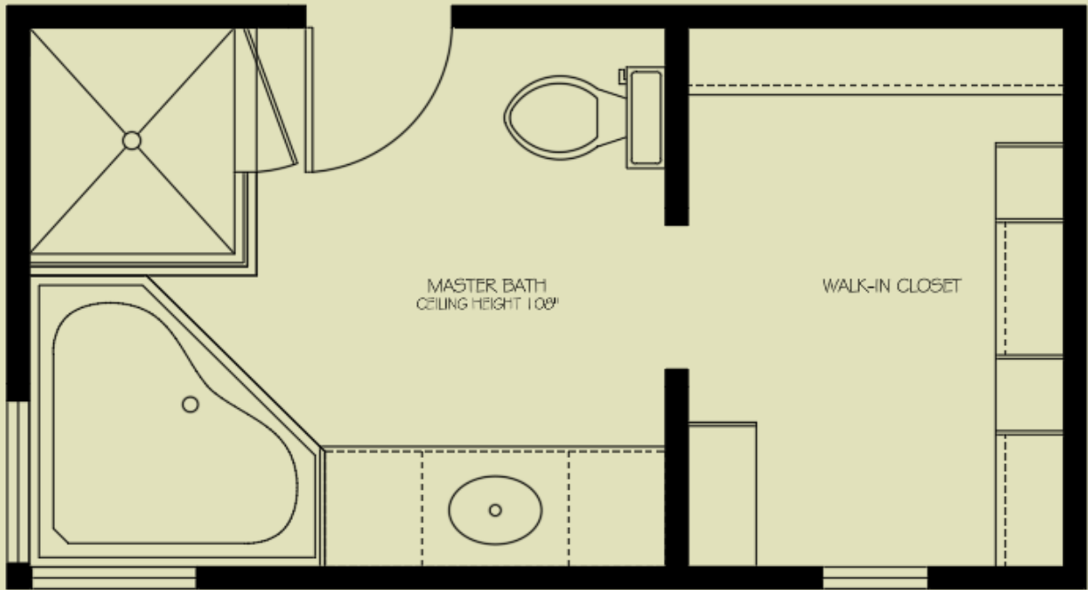
Before Plan
