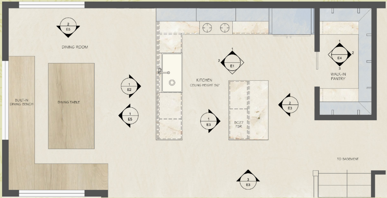
Final Floor Plan in AutoCAD
