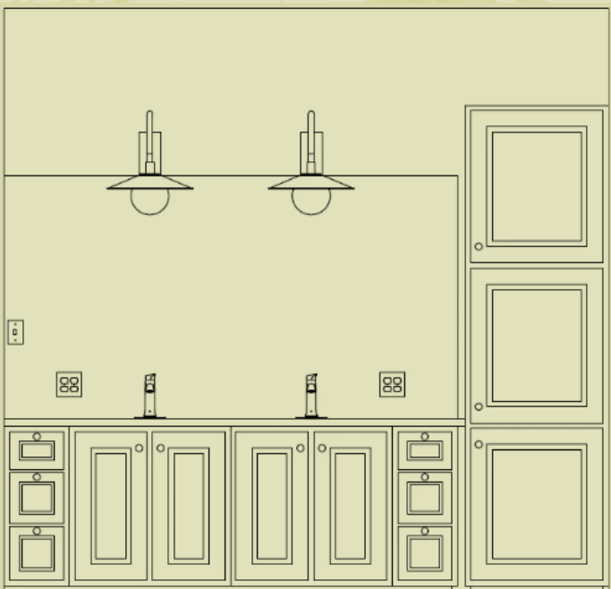
West Elevation
