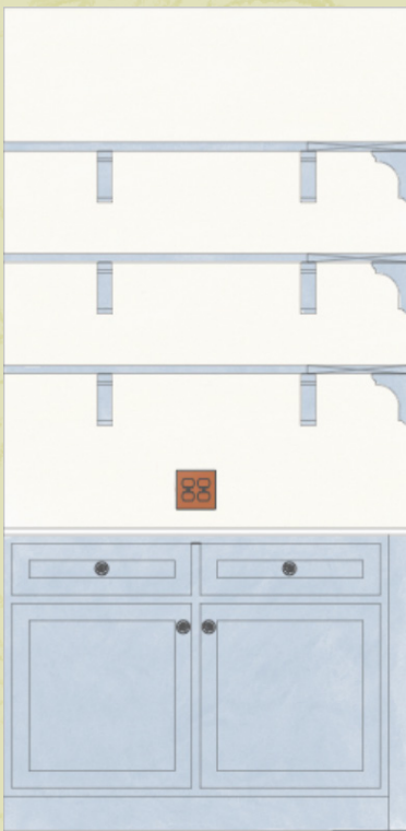
North Elevation
