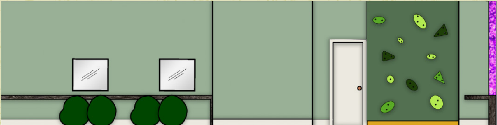
South Elevation
