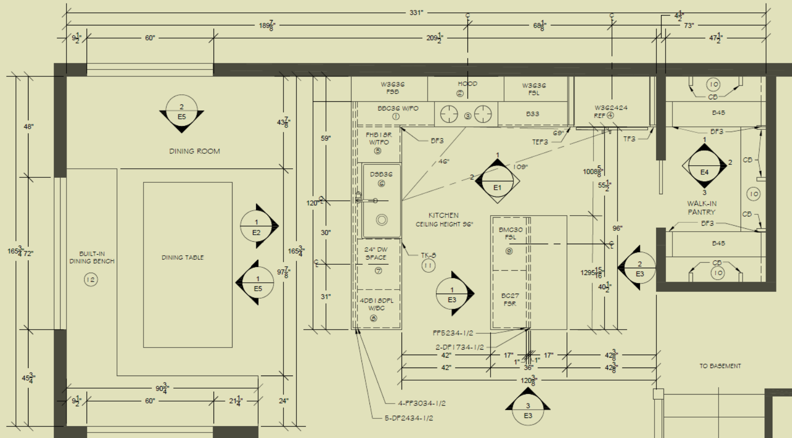
Floor Plan with Nomenclature created in AutoCAD
