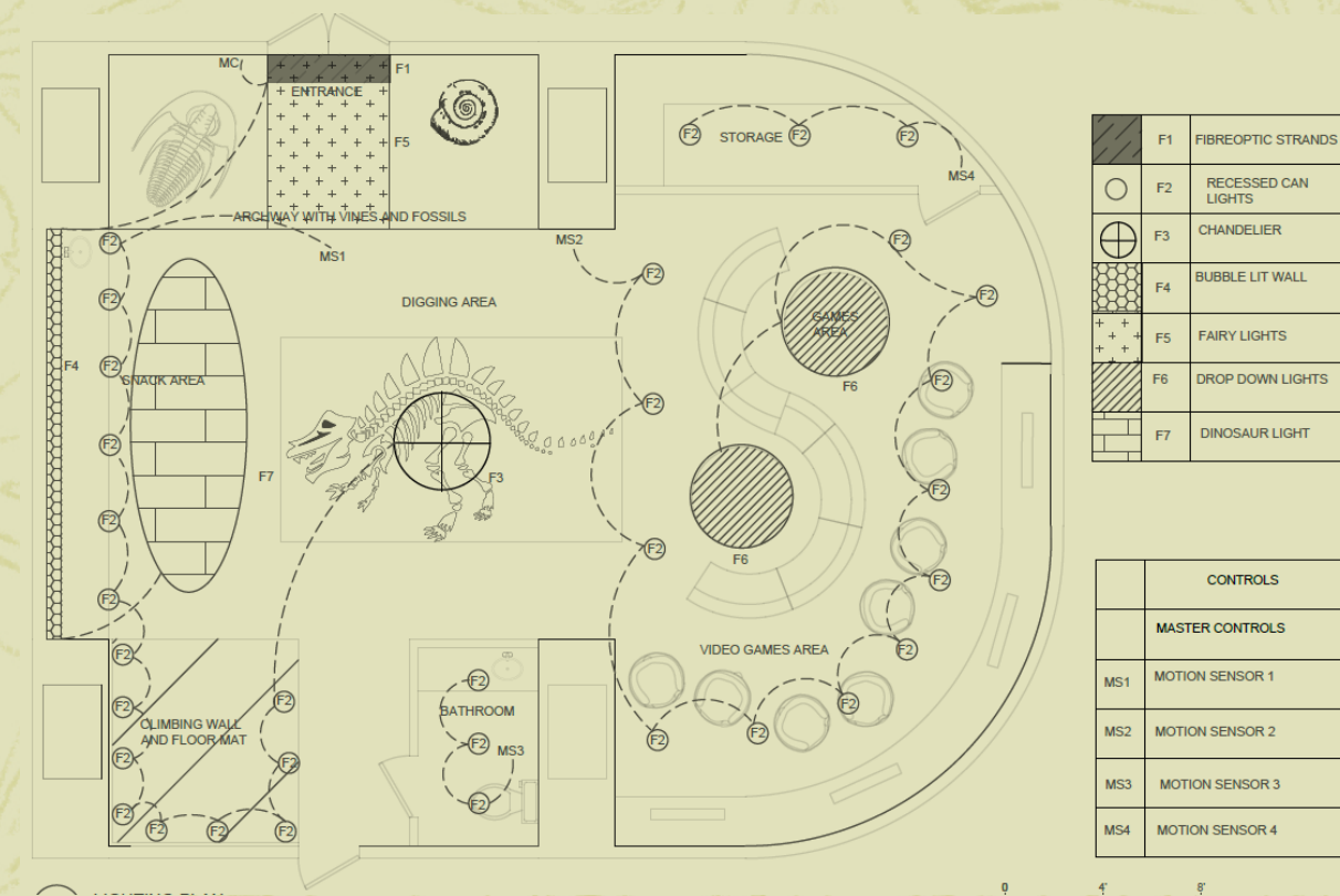
Lighting Plan
